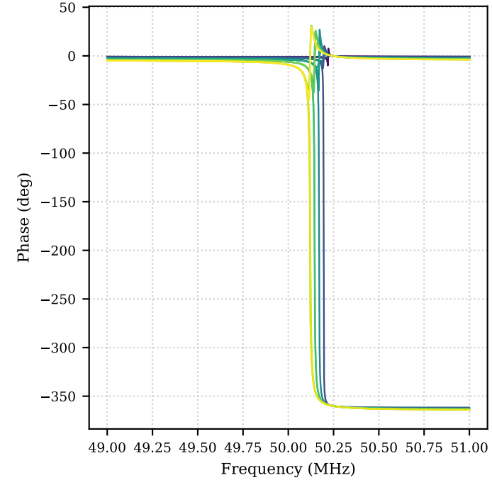
C = 100.32p
