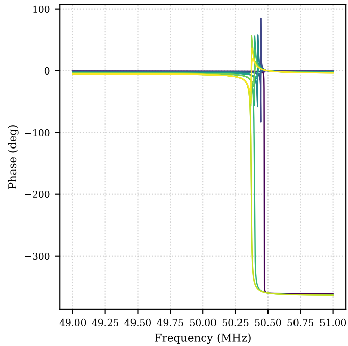
C = 99.32p
