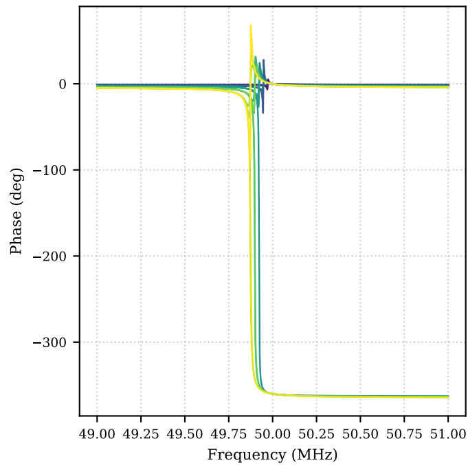
C = 101.32p
